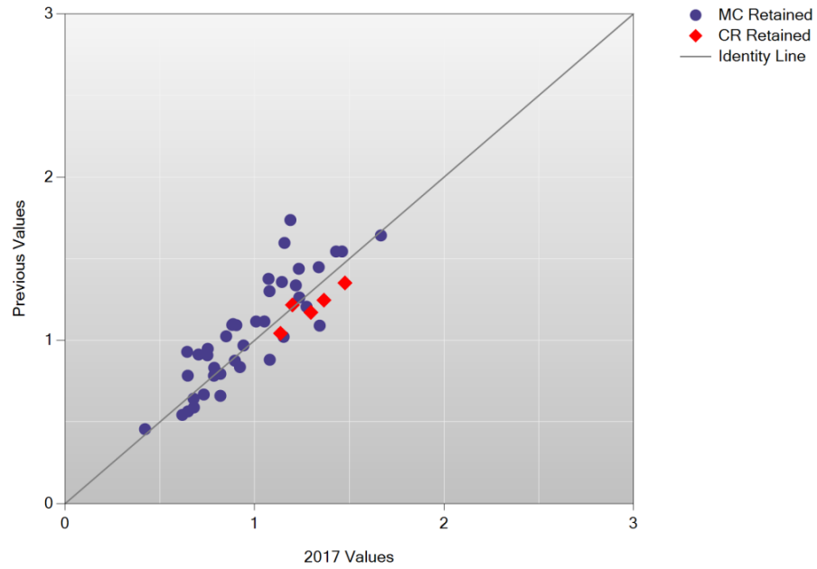
Figure L-14. 2017 Legacy MCAS: b -Plot – Intro to Physics Grade HS
