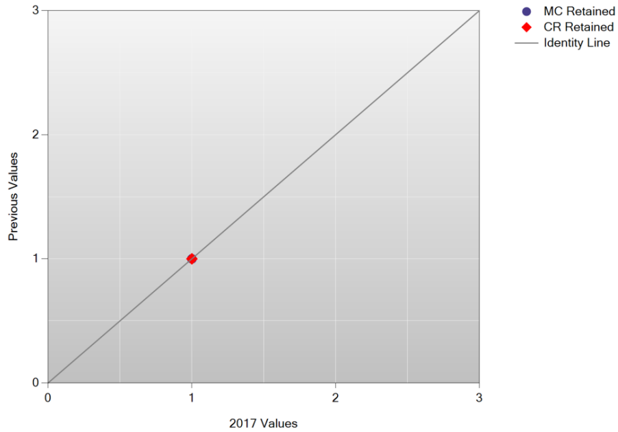
Figure L-16. 2017 Legacy MCAS: b -Plot – Technology and Engineering Grade HS
