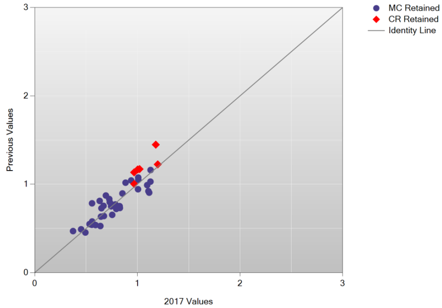
Figure L-2. 2017 Legacy MCAS: b -Plot – ELA Grade 10
